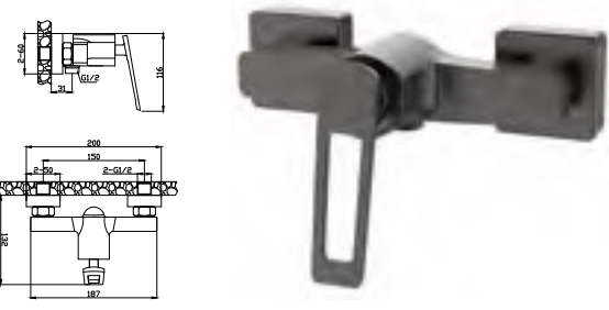
MONOCOMANDO DUCHE TA100/150
