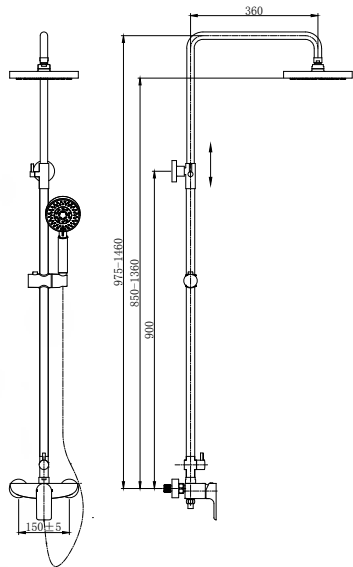
RAMPA MONOC. REDONDA SH300/450 Ref.: RRSTYLE5650CRBLK
